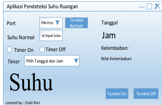
Figure 4. Interface Design
